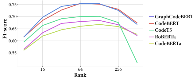
Figure 8: Result of the probe for each model and their best layer according to the dimension of the syntactic subspace for Python. The x axis represents the dimension of the subspace and the y axis the F_1 score.
